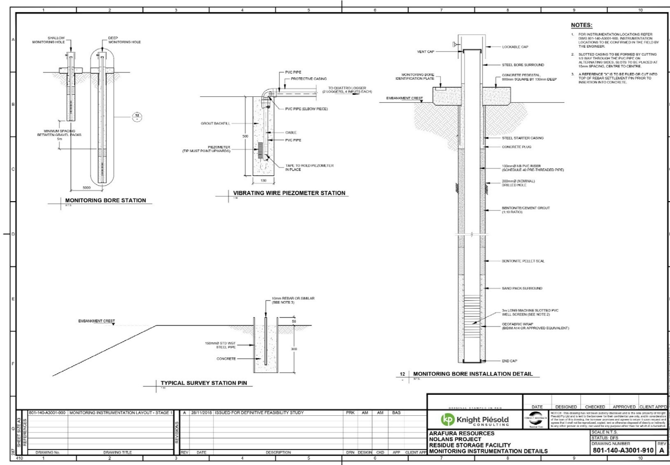
Figure 5-2: Monitoring Instrument Details for the Residue Storage Facility
