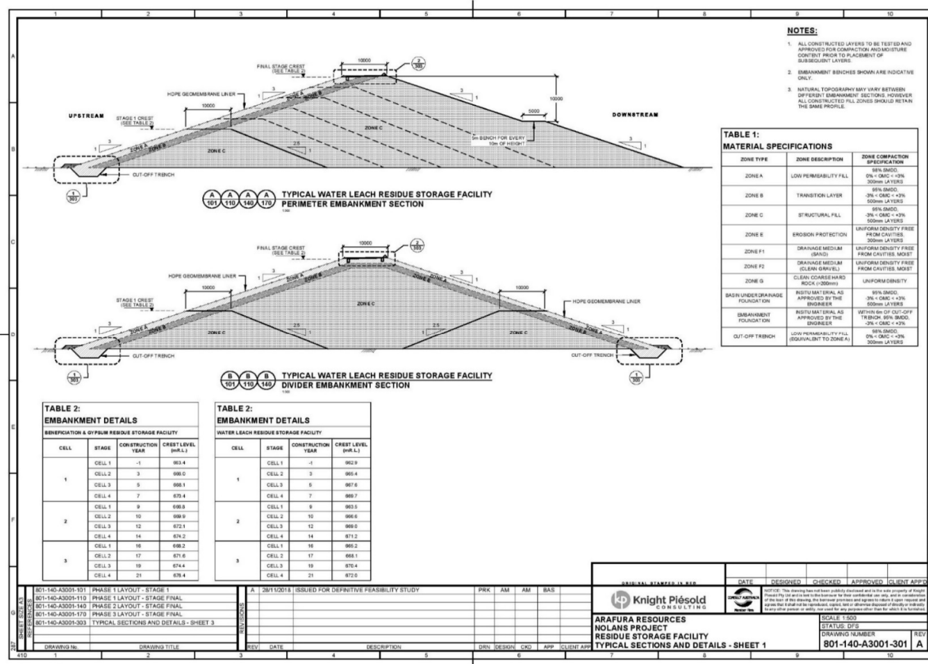
Figure 2-4 Typical Water Leach RSF Perimeter and Divider Embankments Cross Sections
