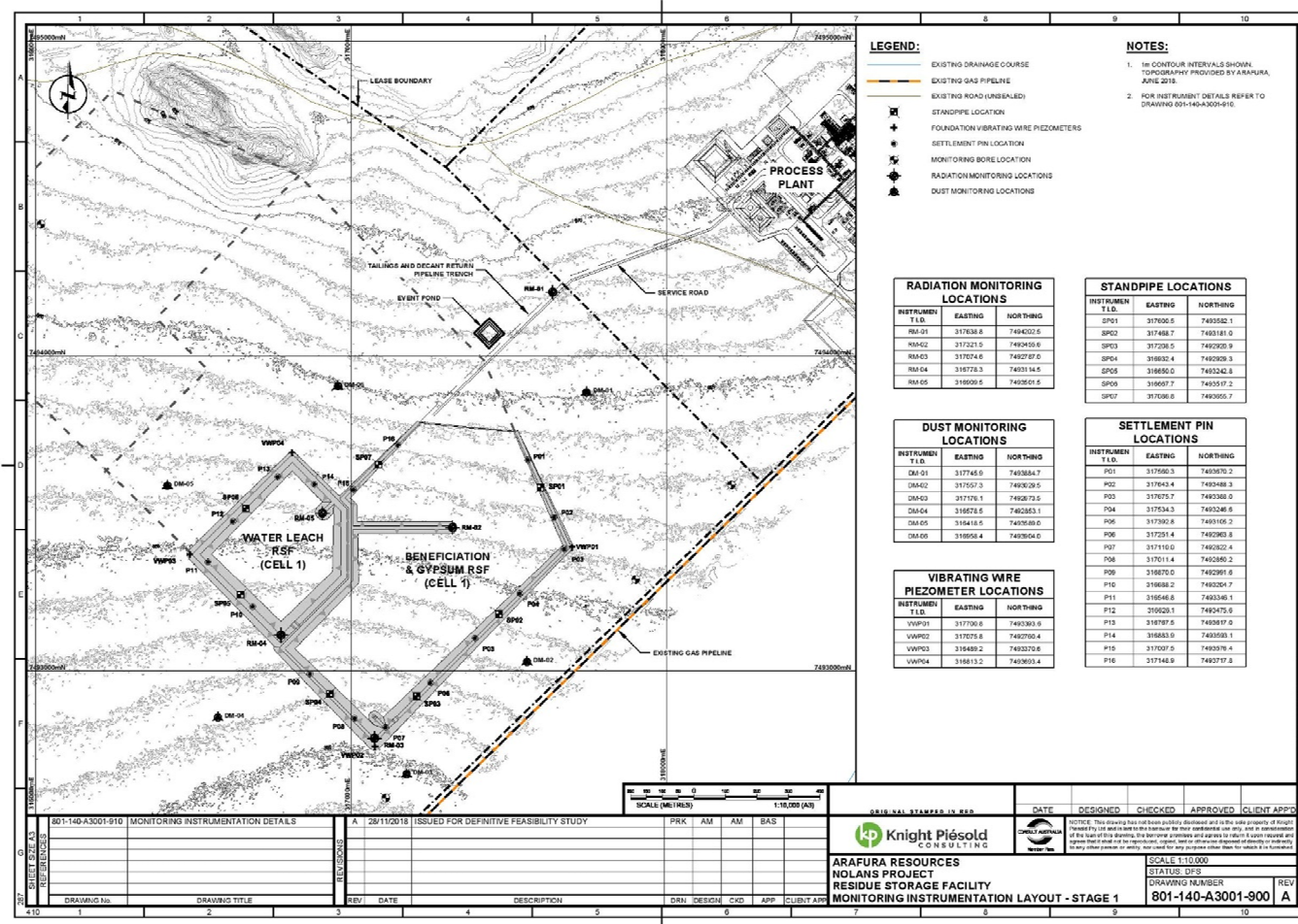
Figure 5-1: Monitoring Instrument Layout for the Residue Storage Facility
