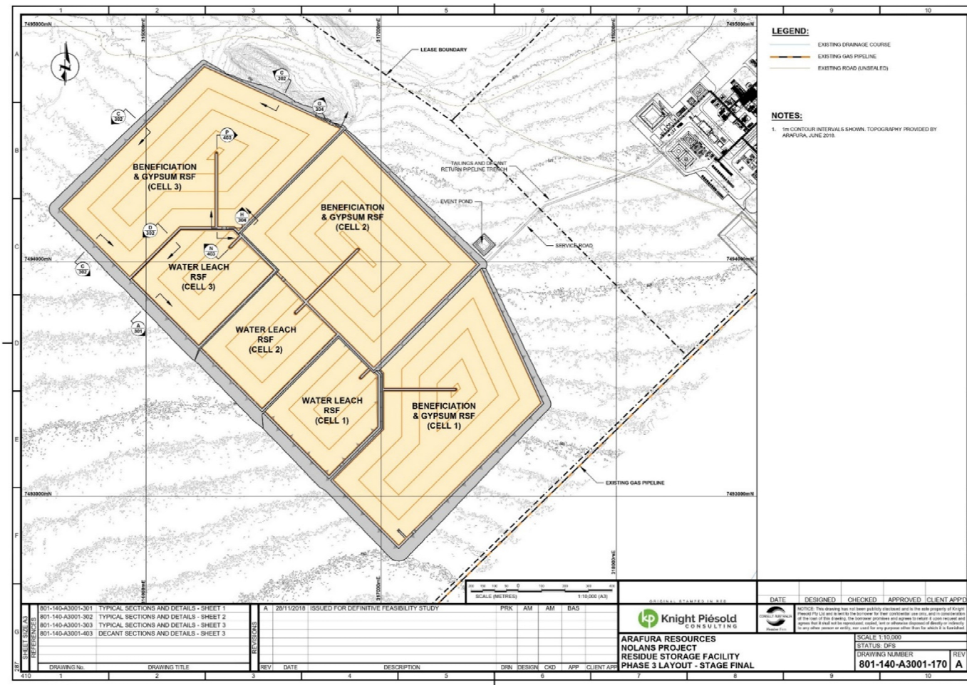
Figure 2-2 : Residue Storage Facility Cell Layout, First 23 years of LOM
