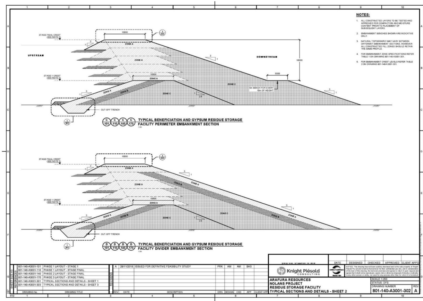
Figure 2-3: Typical Gypsum and Beneficiation RSF Perimeter and Divider Embankments Cross Sections
