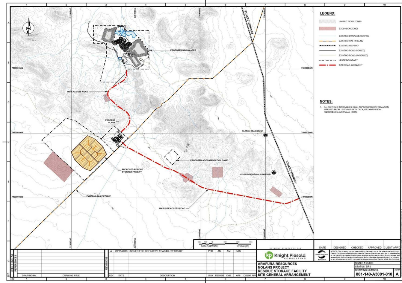
Figure 2-1 : Location of the Residue Storage Facility in Relation to the Site Infrastructure
